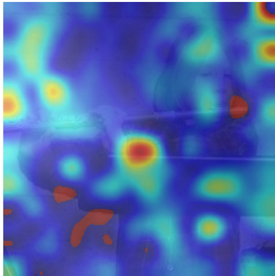
Source(Fog)
